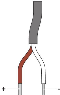
Figure 3 Pin assignment
